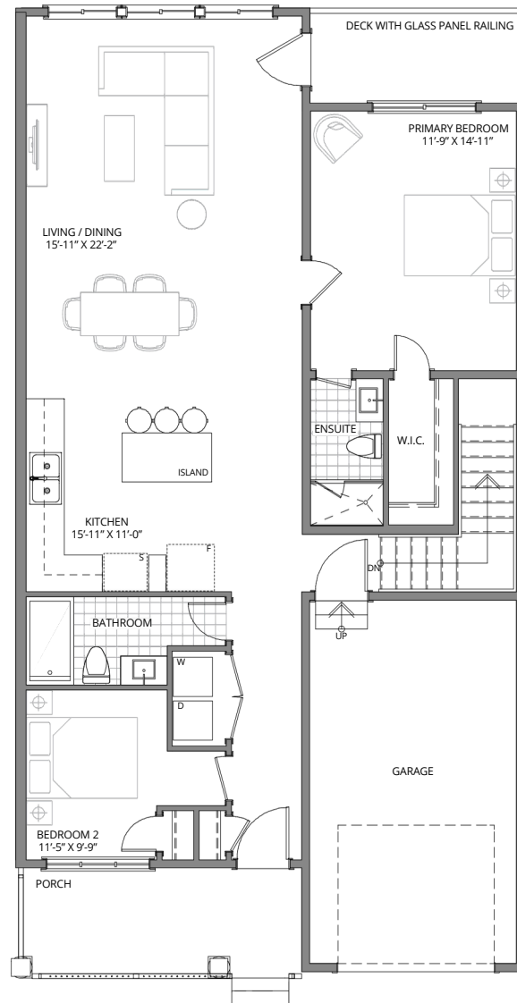
MAIN FLOOR | INTERIOR BUNGALOW TOWN
