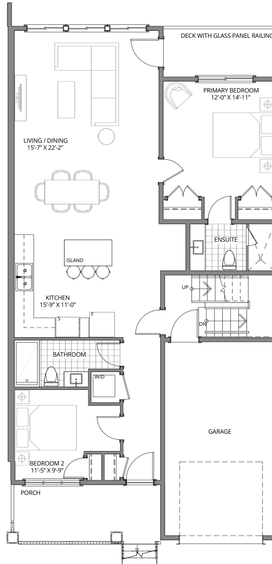
MAIN FLOOR | INTERIOR BUNGALOW TOWN
