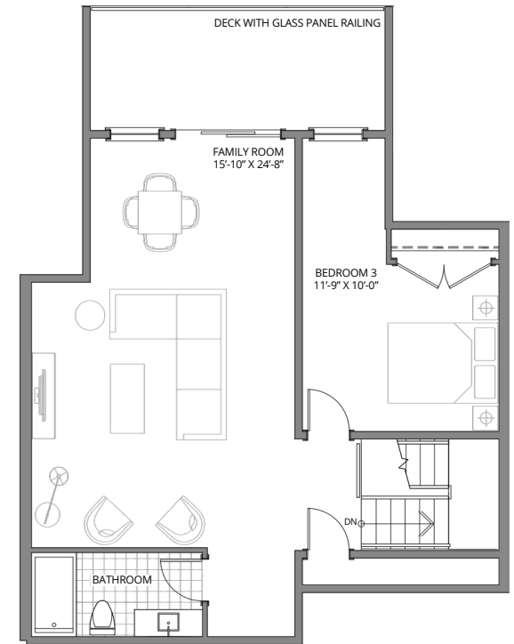
SECOND FLOOR LOFT | INTERIOR BUNGALOW TOWN
